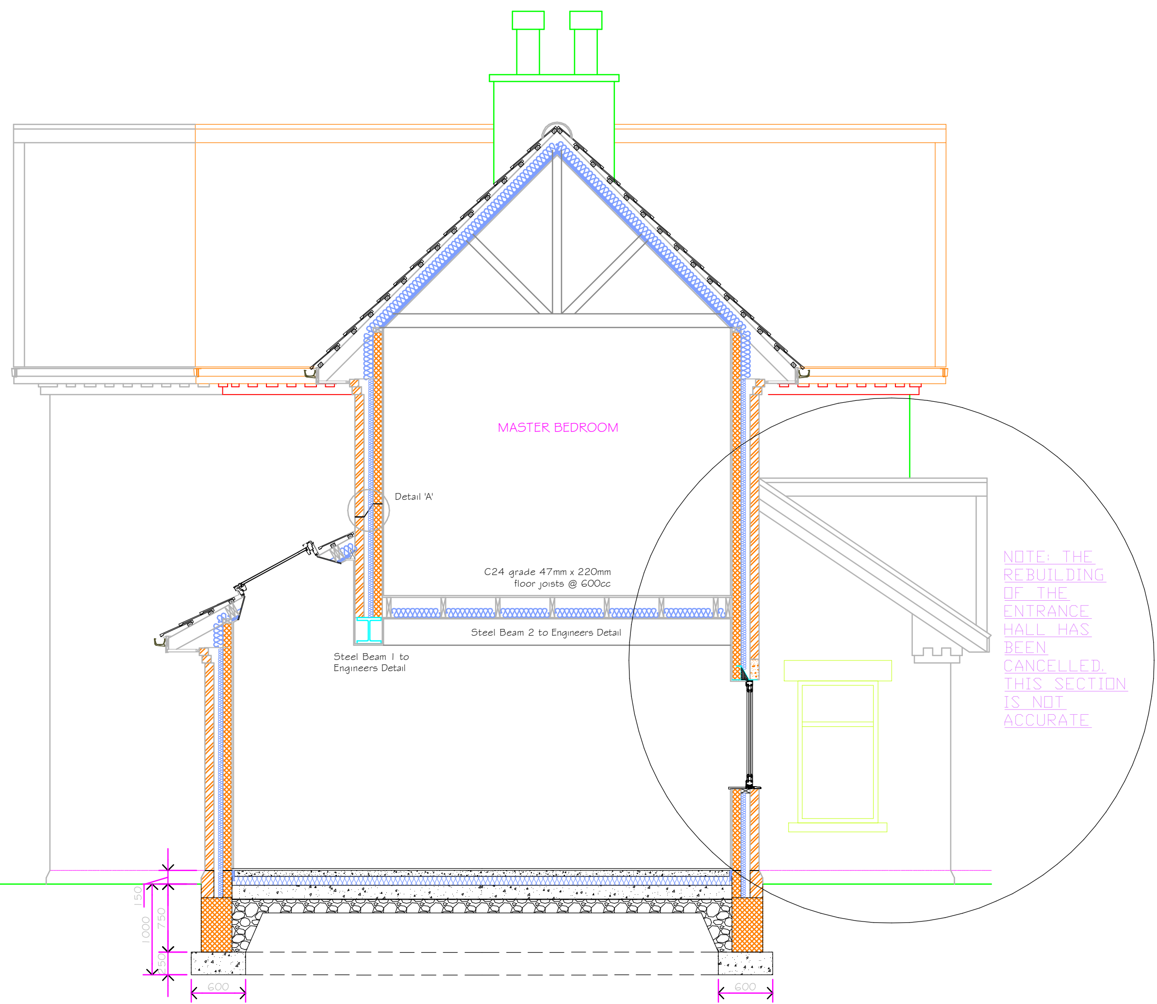
SECTION A-A AS PROPOSED
