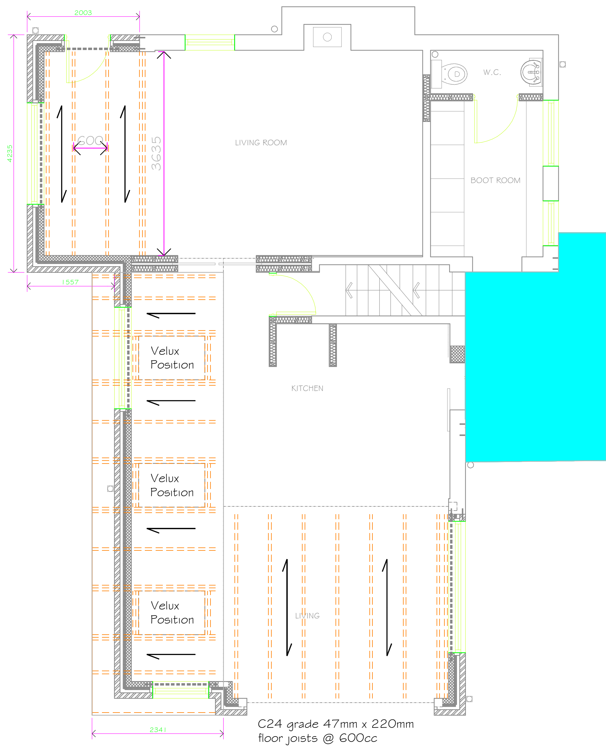
First Floor Joist / Rafter Plan as Proposed
