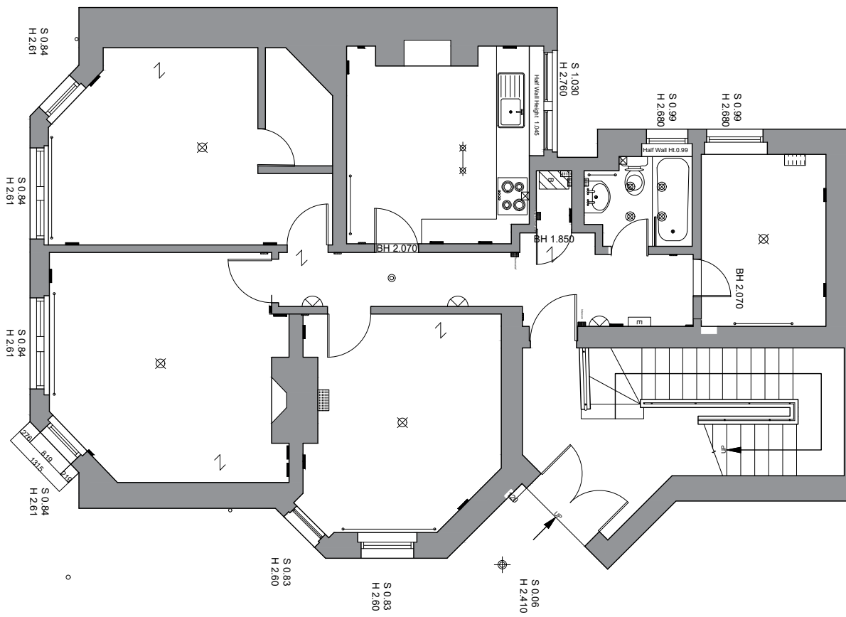
GROUND FLOOR PLAN SCALE : 1:50 ON A3
