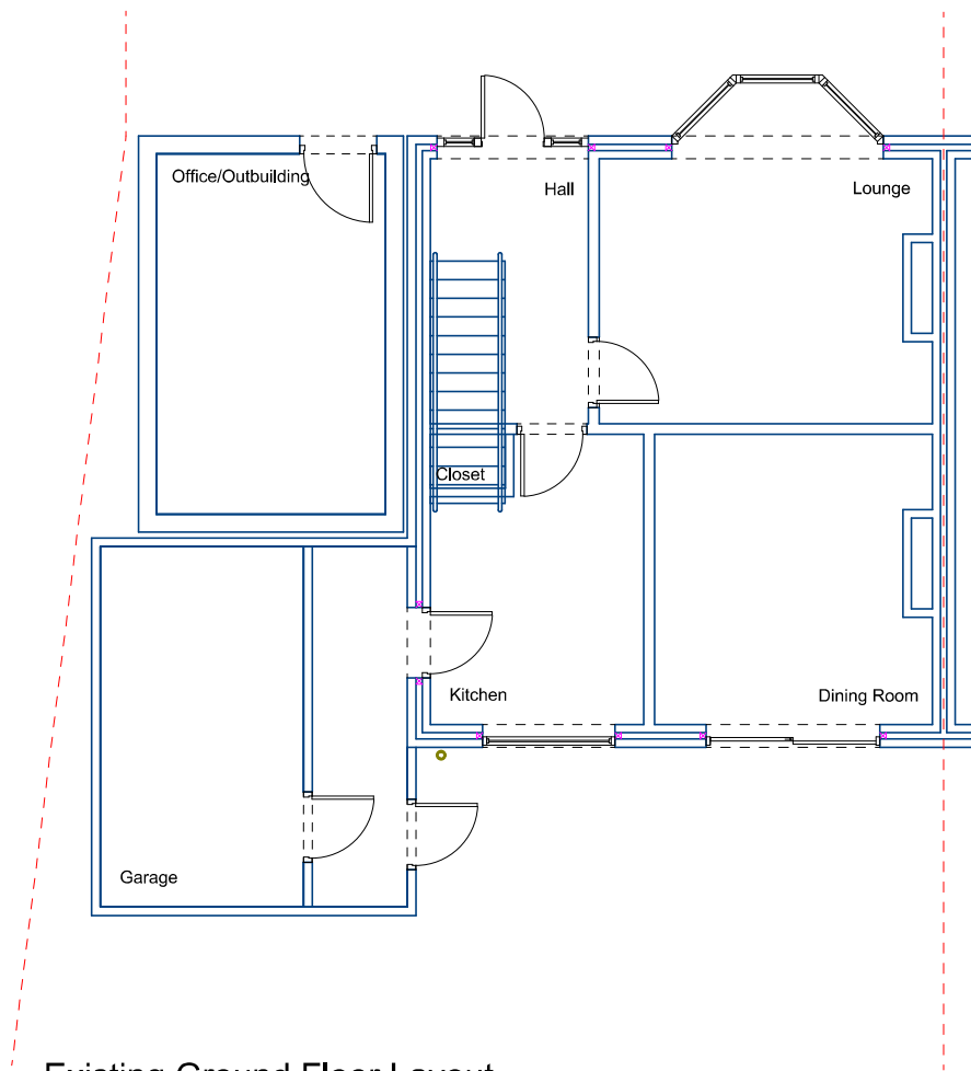
Existing Ground Floor Layout
