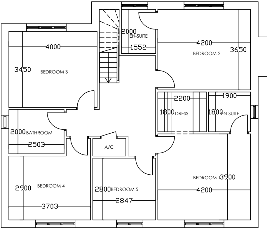
5 BED HOUSE @ 200.8 SQM / 2160 SQFT FIRST FLOOR PLAN SCALE 1:100
