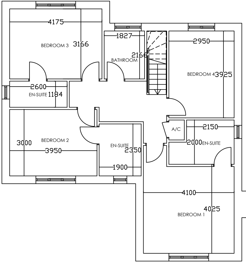
4 BED HOUSE @ 170 SQM / 1829 SQFT FIRST FLOOR PLAN SCALE 1:100
