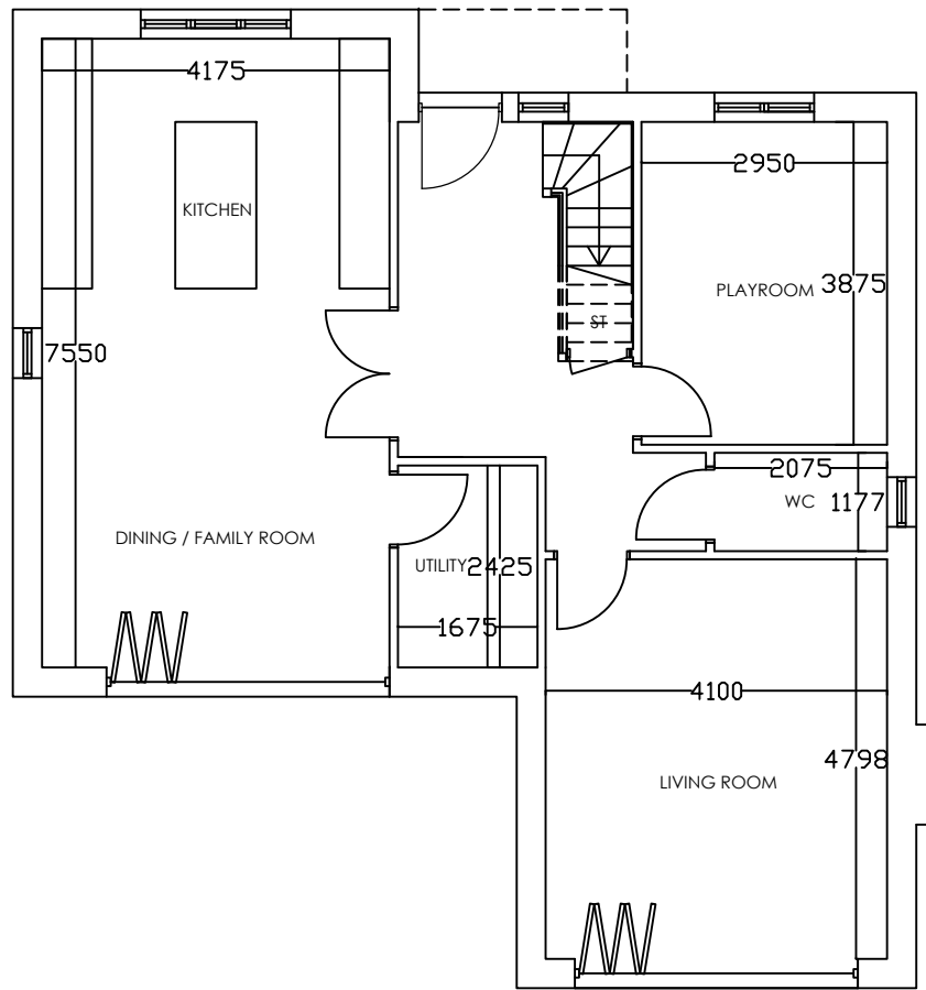
4 BED HOUSE @ 170 SQM / 1829 SQFT GROUND FLOOR PLAN SCALE 1:100
