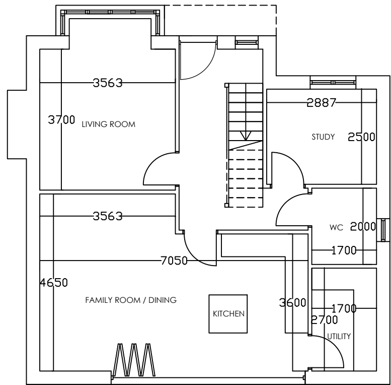
4 BED HOUSE @ 146.6 SQM / 1577 SQFT GROUND FLOOR PLAN SCALE 1:100
