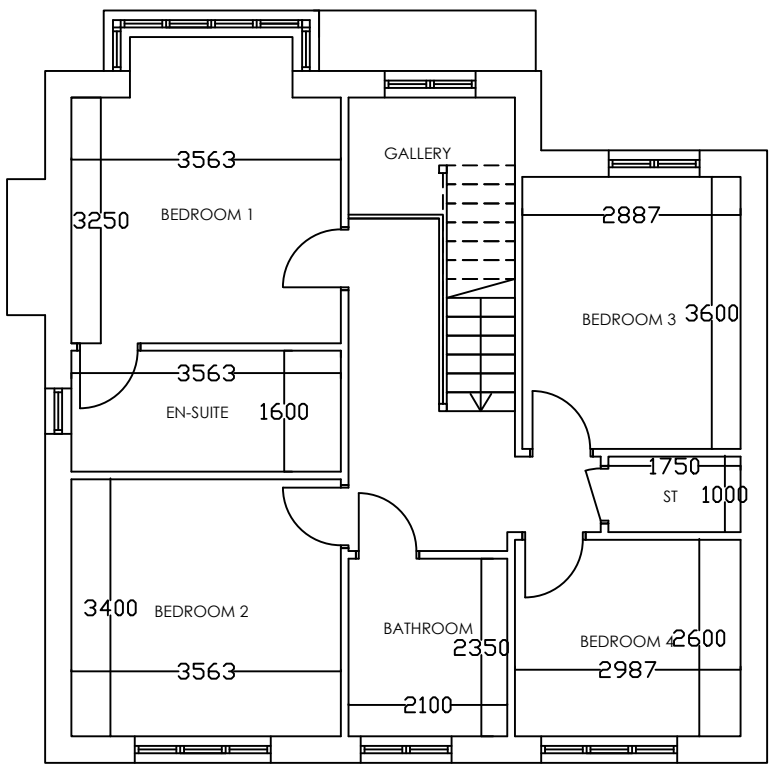
4 BED HOUSE @ 146.6 SQM / 1577 SQFT FIRST FLOOR PLAN SCALE 1:100
