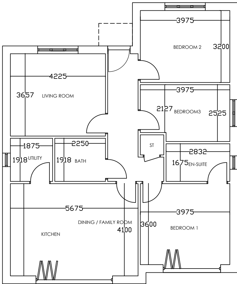
BUNGALOW @ 101.8 SQM / 1095 SQFT FLOOR PLAN SCALE 1:100
