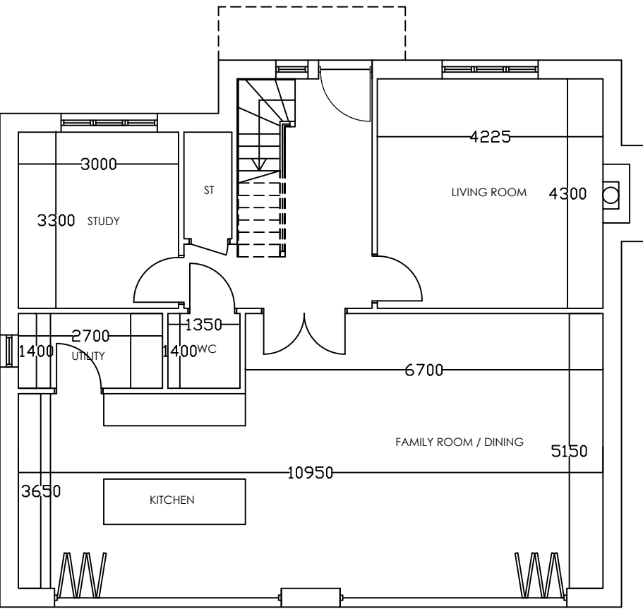
5 BED HOUSE @ 200.8 SQM / 2160 SQFT GROUND FLOOR PLAN SCALE 1:100
