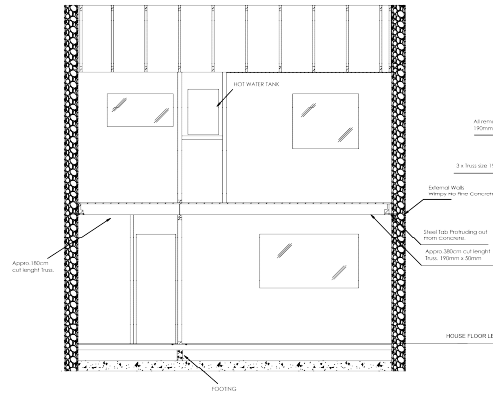
Section View B-B
