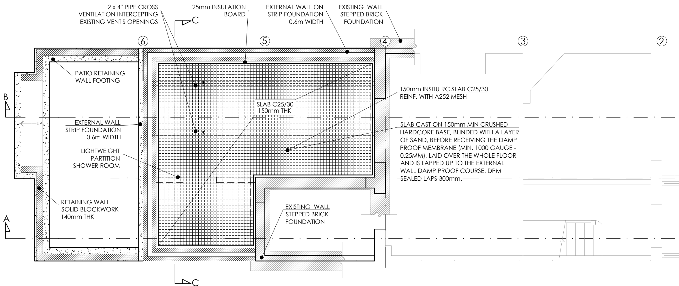
GF STRUCTURES - OPTION 1 'GROUND BEARING SLAB' 1:50
