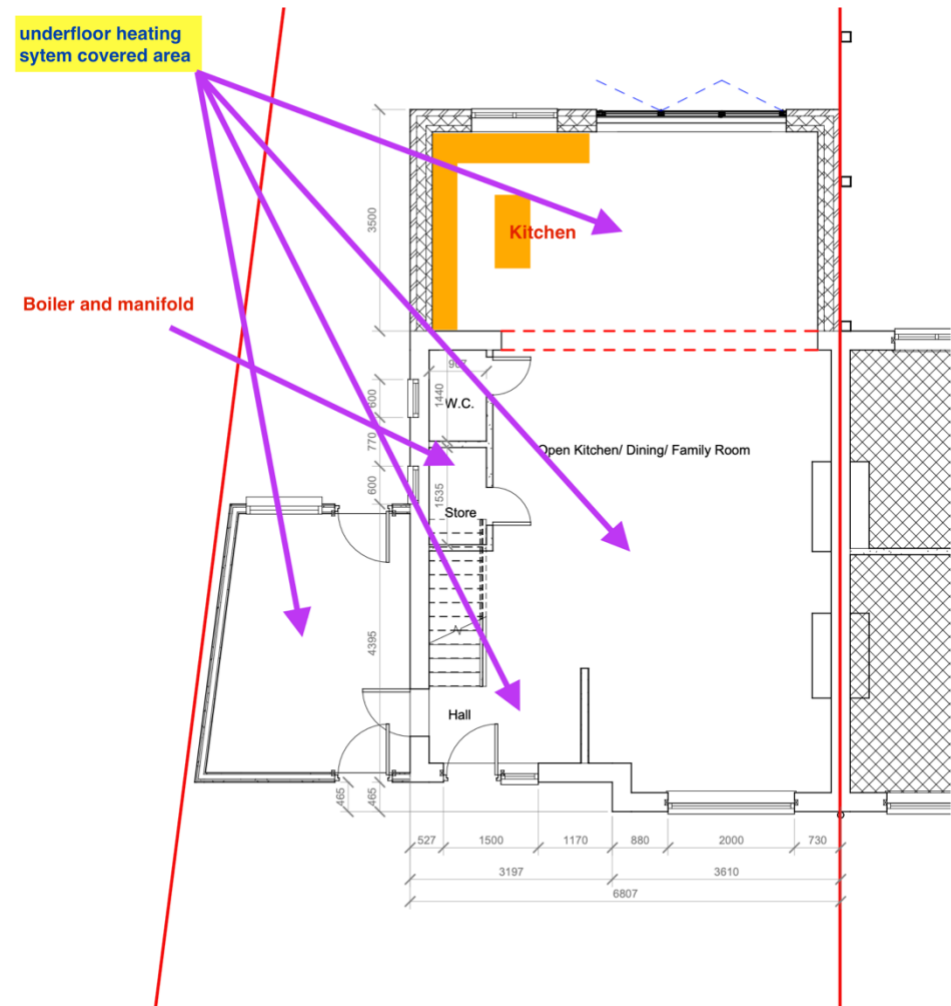
2 Proposed Ground Floor 1 : 50
