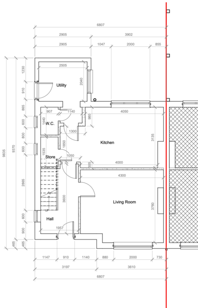
1 Existing Ground Floor 1 : 50
